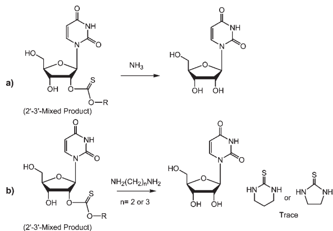
Scheme 8. Complete Cleavage of Thiocarbonates by Exposure to Nucleophilic Amines with Detectable Formation of Ureas or Cyclic Ureas
