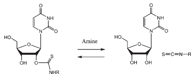
Scheme 9. Elimination of Primary Thionocarbonates To Form Isothiocyanates
