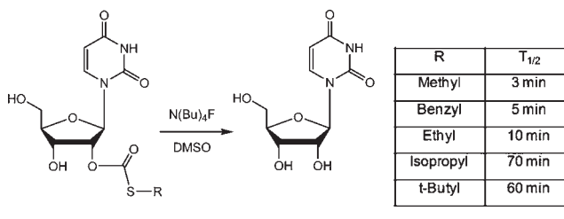
Figure 1. Carbonyl and thionyl 2'-hydroxyl protective group motifs shown to be resistant to 2'→3' migration.
